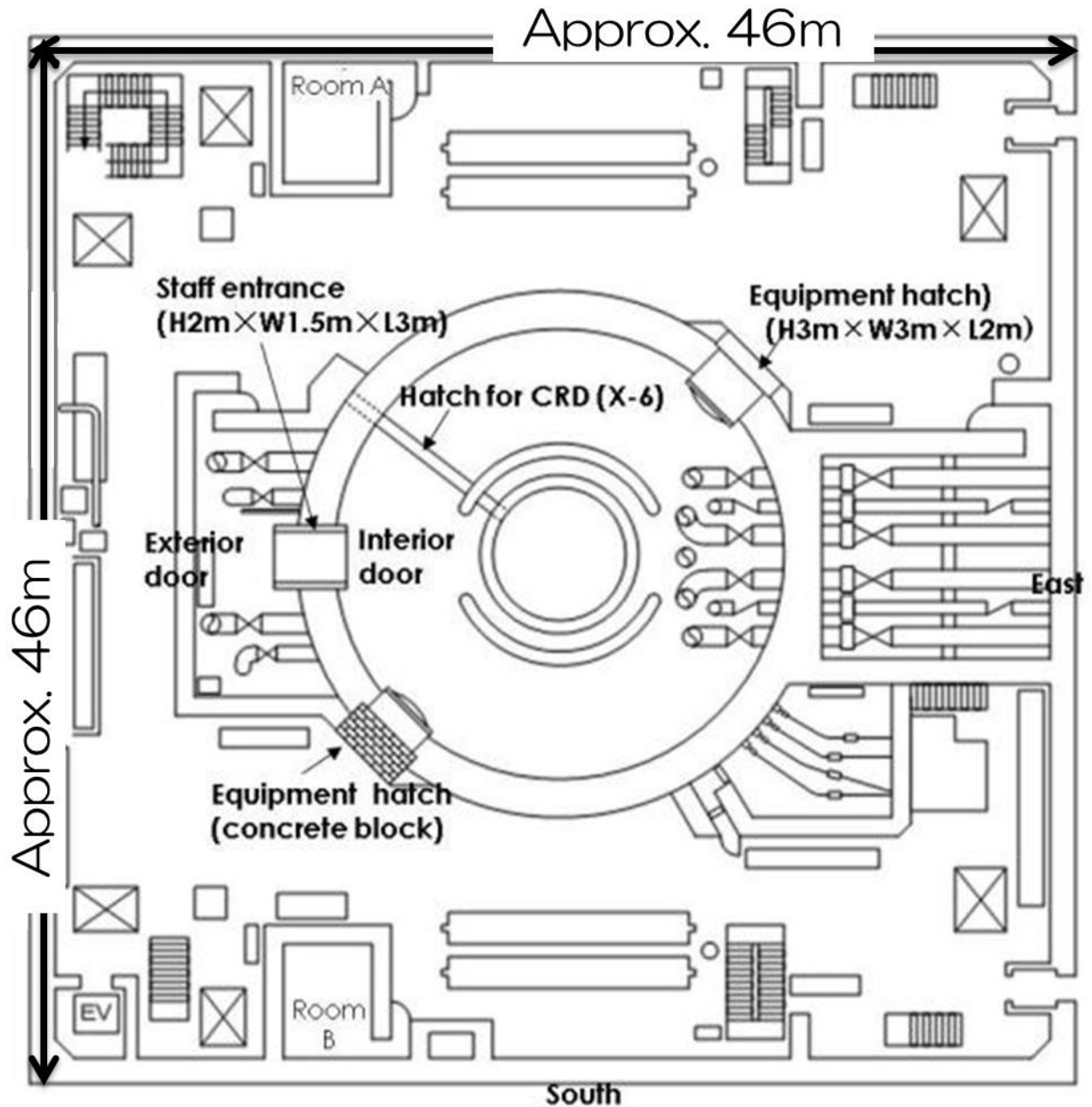
Unit3 R/B 1 st fl.
