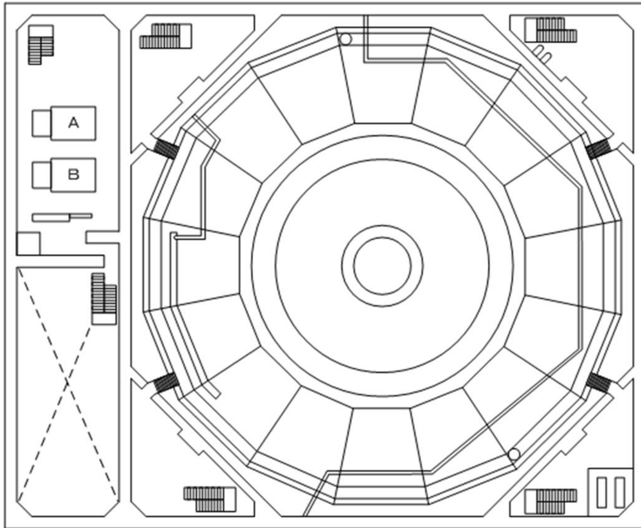
Unit3 R/B Middle Basement fl. 1
