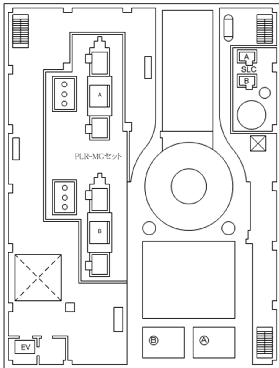
Unit3 R/B 4 th fl.
